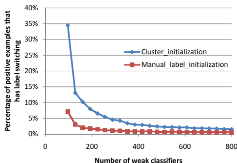
Fig. 2. Percentage of positive examples that switch labels during WTA-McBoost.
