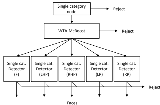
Fig. 5. The three-layer architecture for multi-view face detection. Note in the third layer, the cluster IDs such as F, LHP, RHP, LP and RP are the output of WTA-McBoost and may not represent the true pose of the test window.
