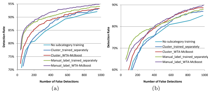
Fig. 4. (a) Performance on CMU+MIT frontal data set (125 images, 483 labeled frontal faces). (b) Performance on CMU profile data set (208 images, 441 labeled faces with various poses, 73 (16.6%) of the faces have more than \pm 10 degree in plane rotations).
