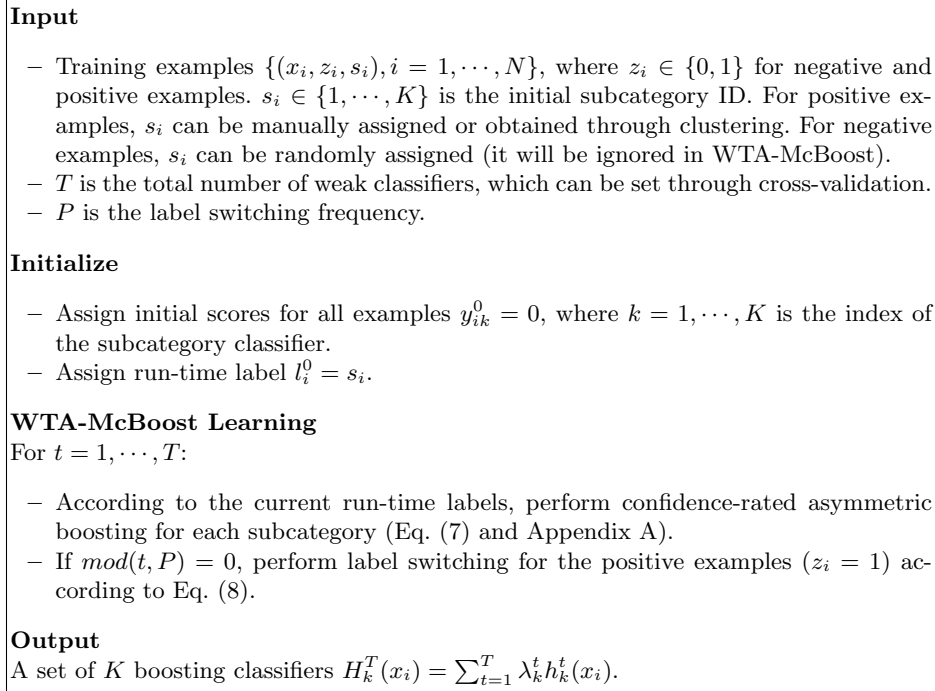
Fig. 1. WTA-McBoost learning.
