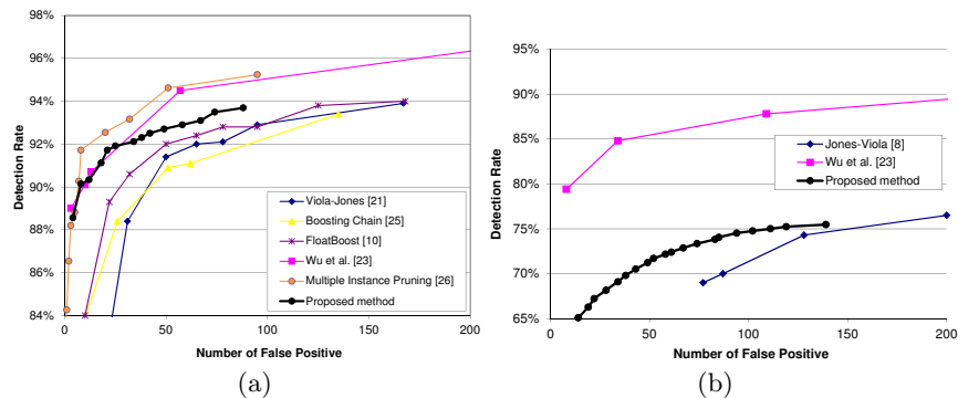
Fig. 6. (a) Performance of our detector on CMU+MIT frontal data set (125 images, 483 labeled frontal faces). (b) Performance on CMU profile data set (208 images, 441 labeled faces with various poses, 73 (16.6%) of the faces have more than \pm 10 degree in plane rotations).
