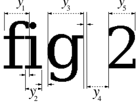
Figure 2. A segmentation of a string of text into 5 primary regions (indicated by the dashed lines) that can be scored for various labelings.
